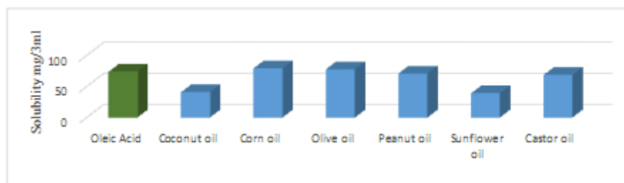
Fig-2: Solubility of Artemisinin in various oils
