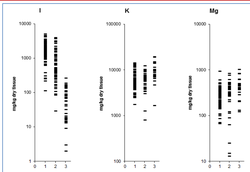
Fig-1: Individual data sets for I, K, and Mg mass fractions in samples of normal thyroid (1), thyroid benign nodules (2) and thyroid malignant nodules (3).
