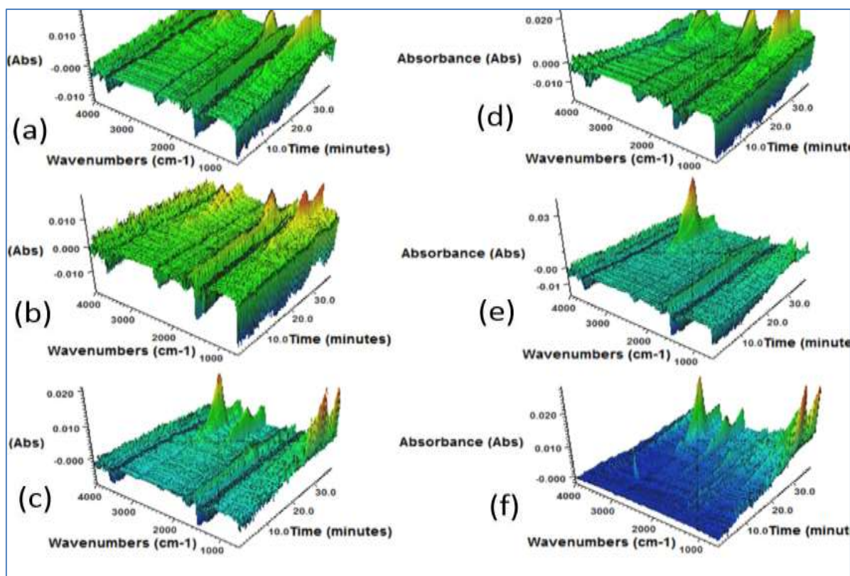
Fig-3: Peak intensity (a) band 940\text{ cm}^{-1} , (b) band 1127\text{ cm}^{-1} , (c) band 1339\text{ cm}^{-1} , (d) band 1380\text{ cm}^{-1} , (e) band 1461\text{ cm}^{-1} and (f) band -1380\text{ cm}^{-1} based on increase in energy level of beam focused on the liquid
