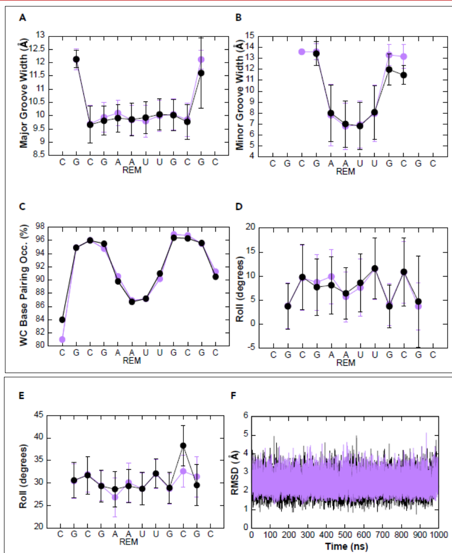
Figure 5: Remdesivir does not distort RNA structure
