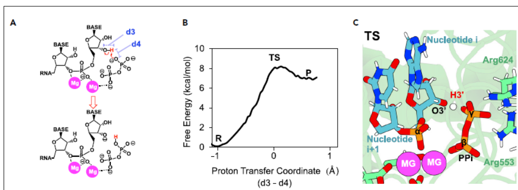
Figure 3: Mechanism of activation through O3' deprotonation inside RdRp
