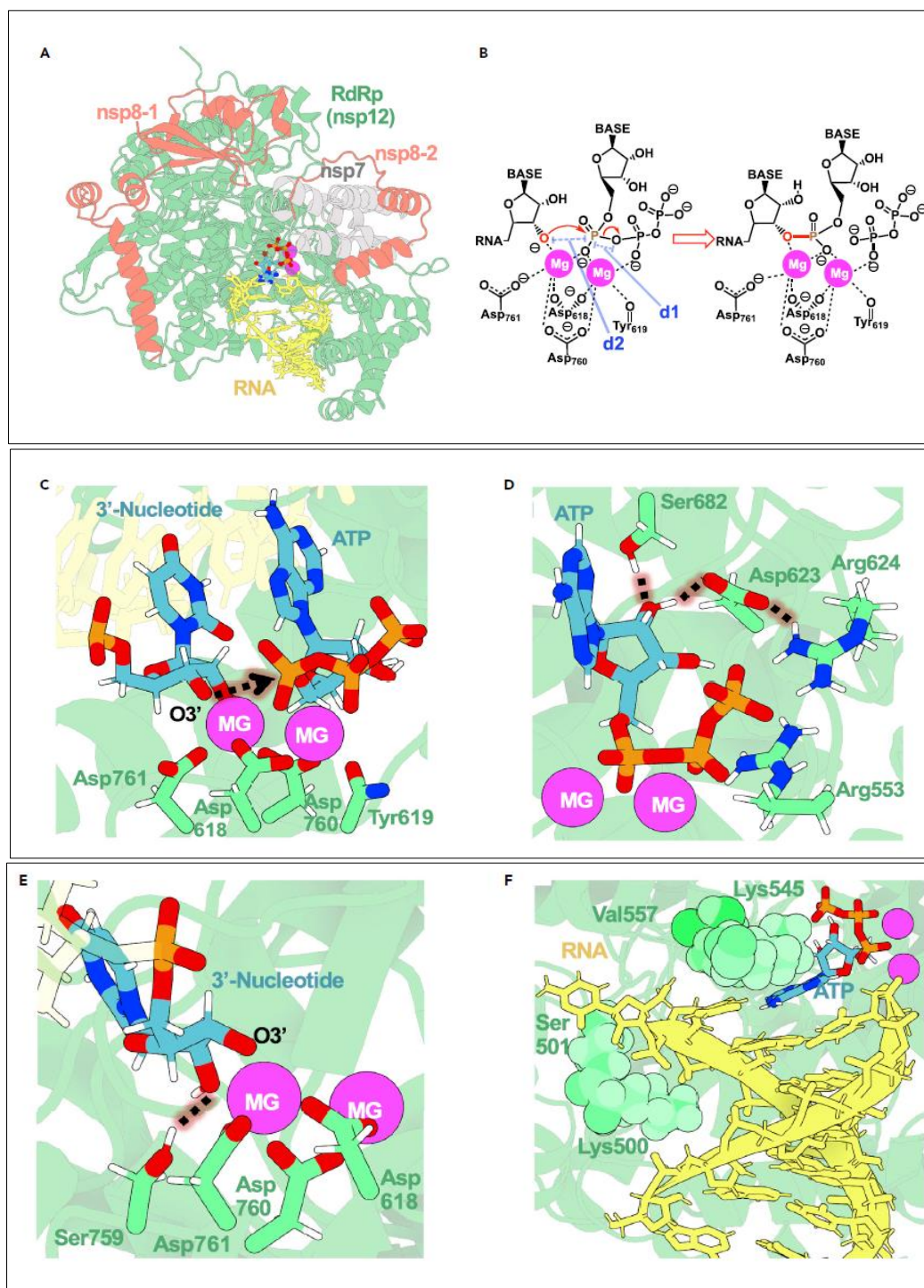
Figure 1: Active site of SARS-CoV-2 RdRp makes it an efficient polymerase
