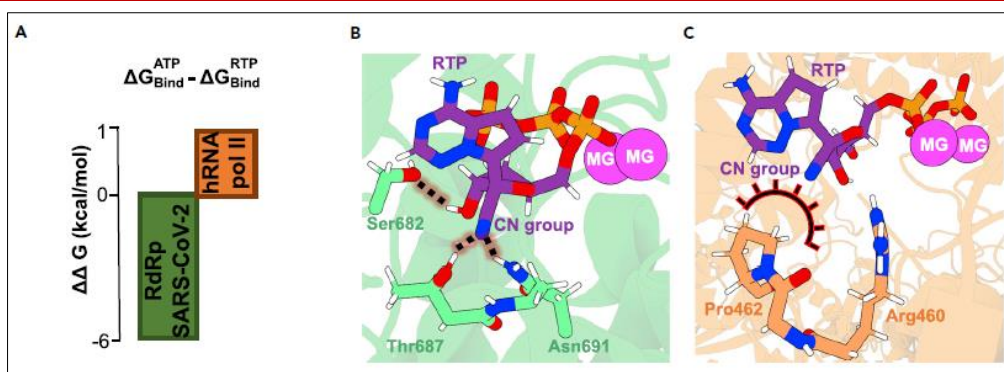
Figure 2: Binding preferences in viral and human RNA polymerases
