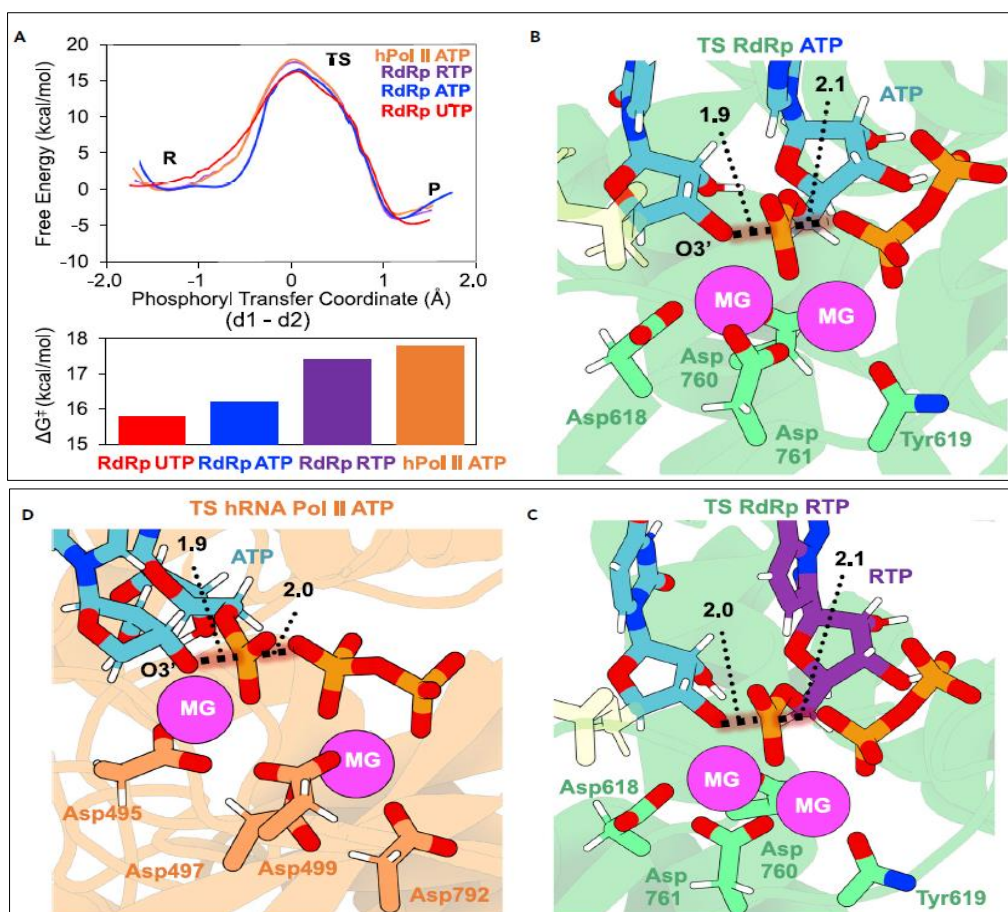
Figure 4: RNA elongation inside RdRp of SARS-CoV-2 and human RNA Pol II
