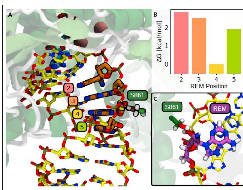
Figure 6: Remdesivir elongation along RdRp's exit channel
