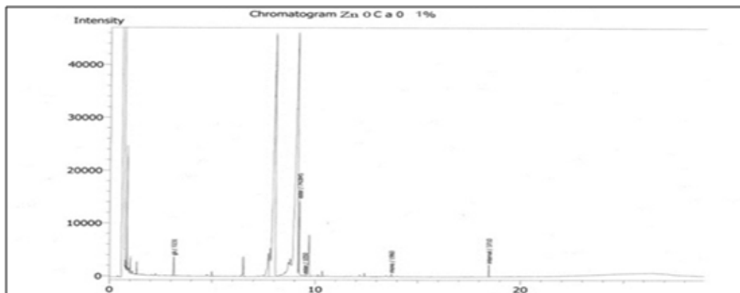
Fig-2: Chromatogram GC Analysis of Transesterification Result of Avocado Seed Oil with ZnO / CaO catalyst with ZnO loading 1%
